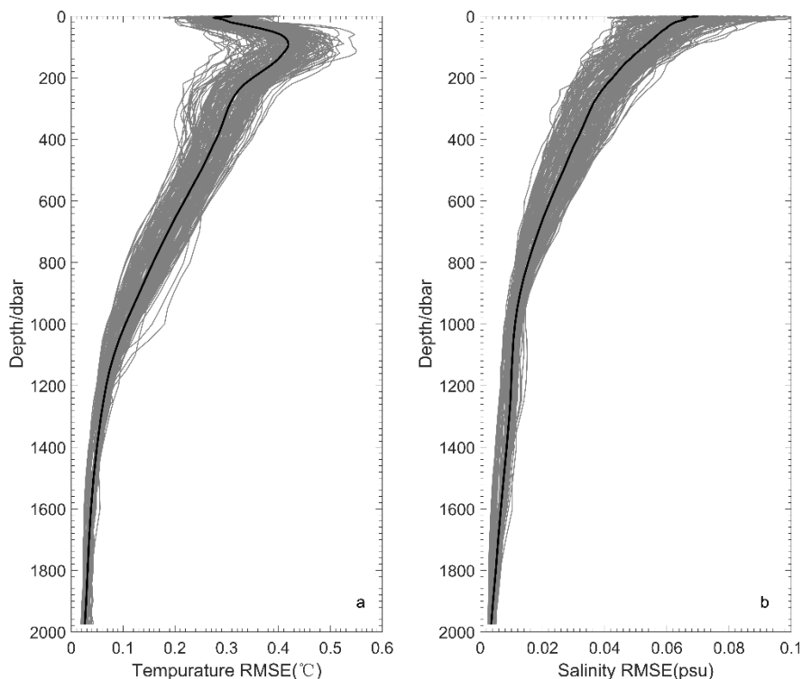
Figure 3 RMSEs of (a) temperature and (b) salinity between the gridded BOA_Argo analysis and merged observations after the objective analysis step (January 2004–December 2017). Solid black line denotes the average value of RMSEs for each variable, while solid grey lines denote the monthly RMSEs over the global oceans.
