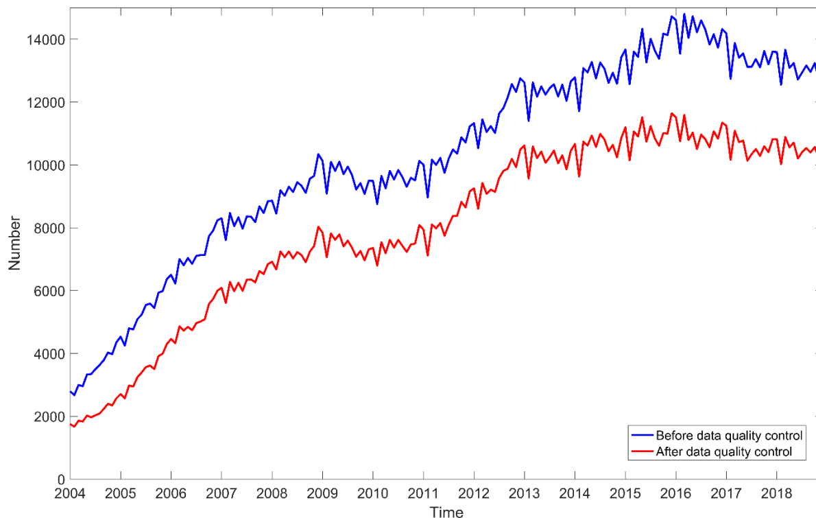
Figure 2 Number of Argo profiles before (blue) and after (red) a data screening from January 2004 to December 2018.
