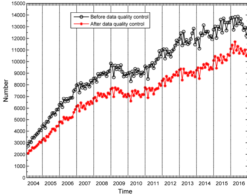
Figure.2 Number of Argo profiles before (black) and after (red) a data screening from January 2004 to December 2016.
