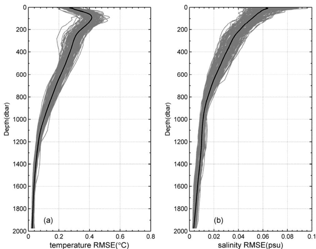
Figure.3 RMSEs of (a) temperature and (b) salinity between the gridded BOA-Argo analysis and merged observations after the objective analysis step (January 2004–December 2016). Solid black line denotes the average value of RMSEs for each variable, while solid grey lines denote the monthly RMSEs over the global oceans.
