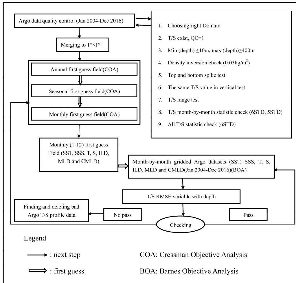
Figure.1 Scheme describing the production of the BOA-Argo gridded data set, including quality control and preprocessing of Argo data, as well as iterative applications of the objective analysis and RMSE check steps.
